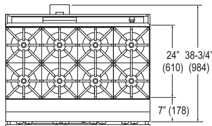
TOP VIEW 2" (51)
